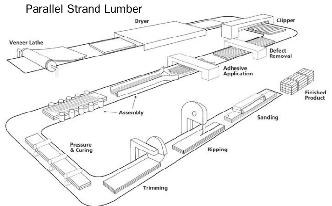
Figure 5 Parallel Strand Lumber Manufacturing Process
