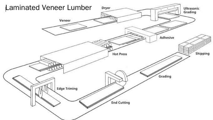
Figure 6 Laminated Veneer Lumber Manufacturing Process
